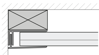
FCD201 Two Part Universal Edge Trim
