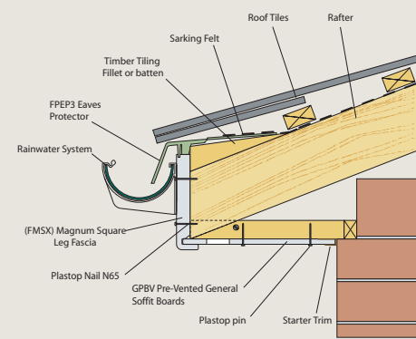
Fig 5. Magnum Xtra Square Leg Fascia with horizontal soffit.
