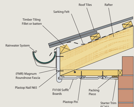
Fig 20b. Wide soffit application using Open V cladding profile.
