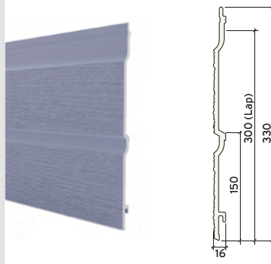
DOUBLE PLANK SHIPLAP CLADDING (FCD300E)
