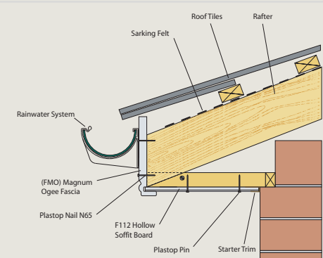
Fig 8. Magnum Ogee Fascia with horizontal hollow soffit.
