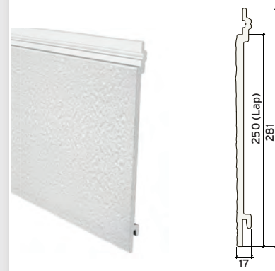
FLAT PANEL CLADDING (FCP250E)*
