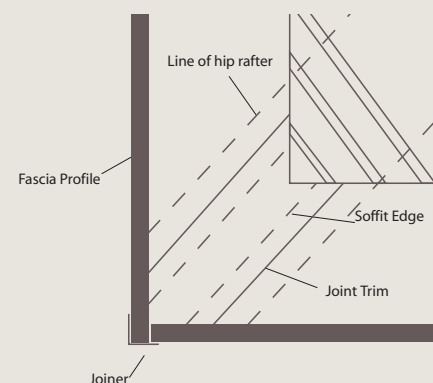
Fig. 20d. Soffit Corner detail showing soffit returns, corner trim, etc.
