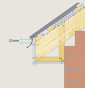
25mm Air gap* ***Duo pitch roof with insulation following plane of roof
