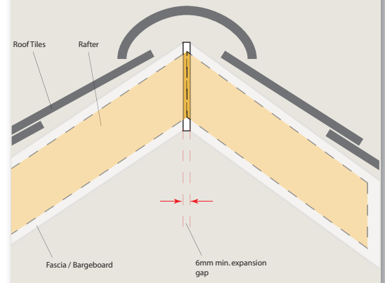
Fig. 22 Bargeboard at gable end showing apex.
