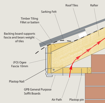
Fig. 19 Refurbishment of pitched roof eaves and soffit, incorporating ventilation.
