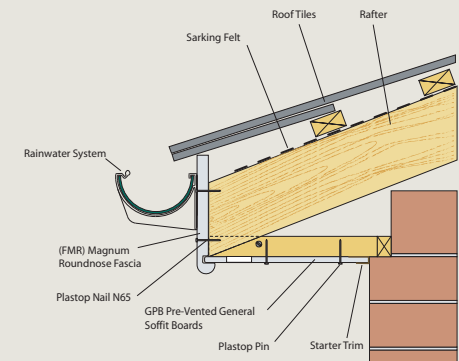
Fig 6. Magnum Roundnose Fascia with horizontal soffit.
