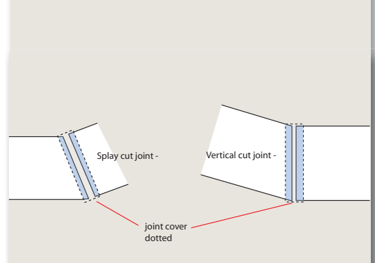
Fig. 23b Junction of fascia with In-line gable.
