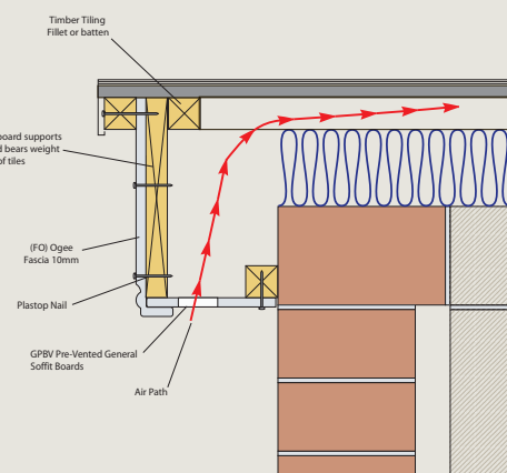
Fig. 20 Refurbishment of flat roof eaves and soffit, incorporating ventilation.
