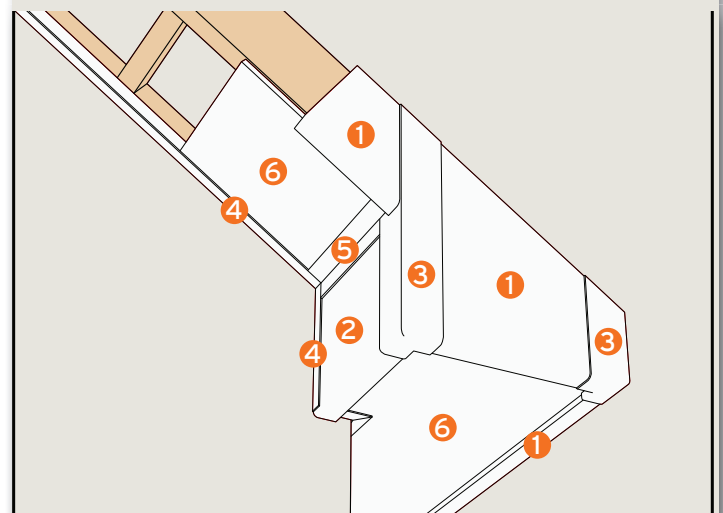
Fig. 25. Magnum Roundnose Fascia box end with splay cut junction.
