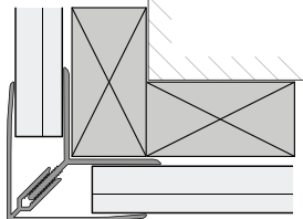
FCD204 Two Part Corner - External
