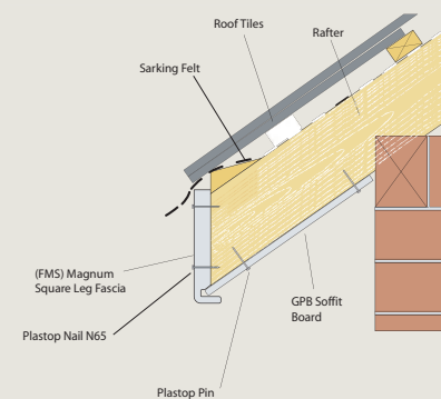
Fig 20c. Inclined soffit application with GPB soffit.
