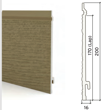
WEATHERBOARD CLADDING (FCF170E)
